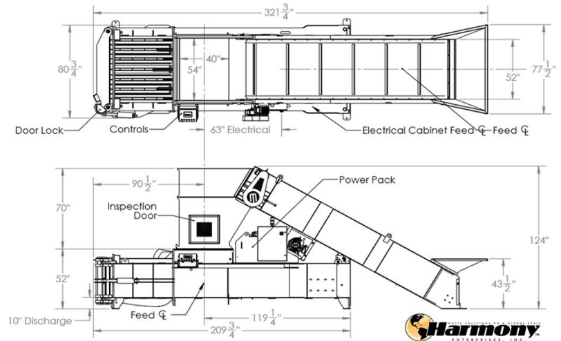
Harmony HM-60 Closed Door Manual Tie Baler
