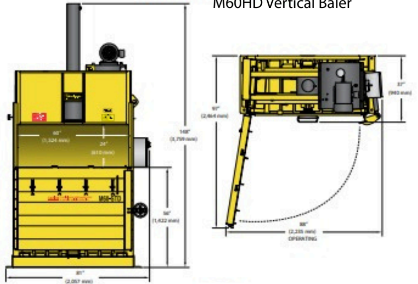
M60HD Vertical Baler
